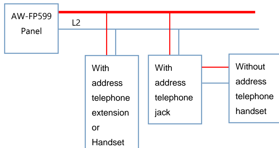
Fig. 23 Wiring diagram of supporting equipment
