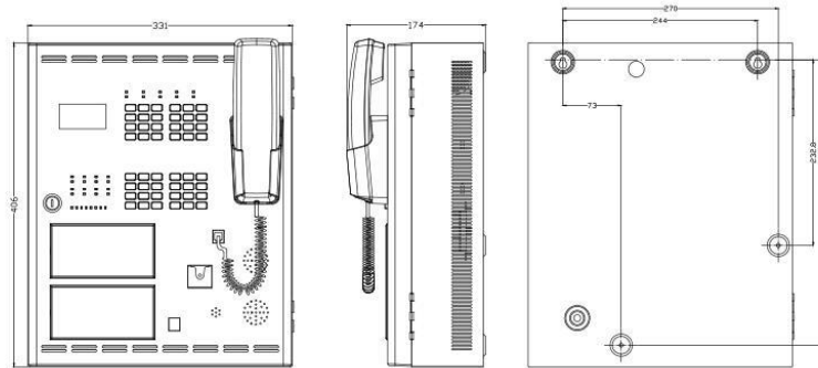
Fig. 4 Dimensions of chassis
