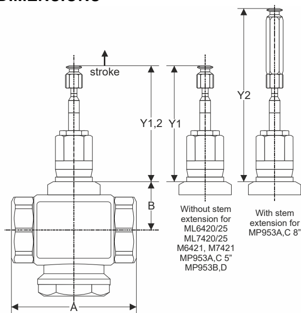
Fig. 1. Dimensions (2-port)
